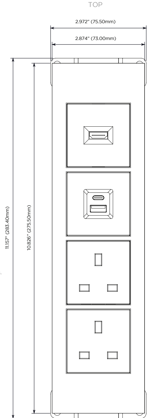
Shown with 2 "Type G" 220 VAC Tamper Resistant ACs, 1 USB-A & USB-C Charging Port, and 1 HDMI Port.
